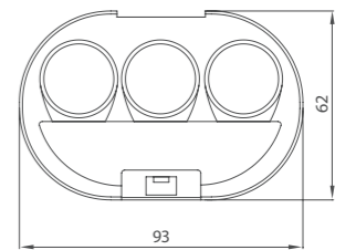
Shadows ILLU17006 3 hole palette 3ml * 3
