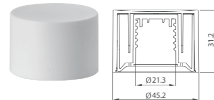
Over cap DRA-skin ILLU16004
