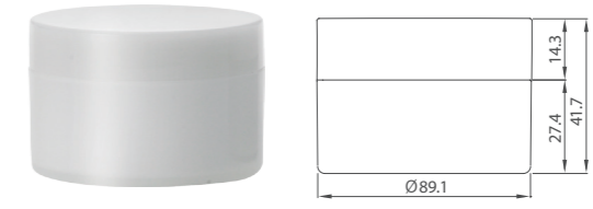
Cream Jar Double injection 200ml ILLU11004
