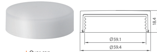
Over cap DP-cream ILLU16002
