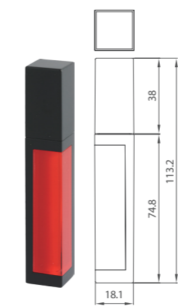
Lipgloss Double Injection S2 Type 3ml ILLU12012
