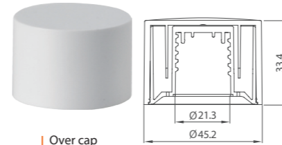
Over cap DDA-skin ILLU16005
