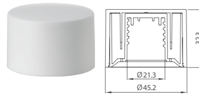
Over cap DSA-skin ILLU16003
