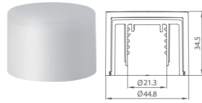
Over cap DP-skin ILLU16001
