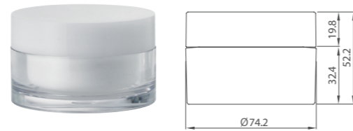
Cream Jar Double containe 50ml ILLU110014
